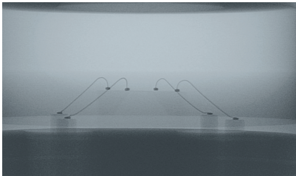
Figure 1. X-ray of die and wire bonds after gel dispense.
